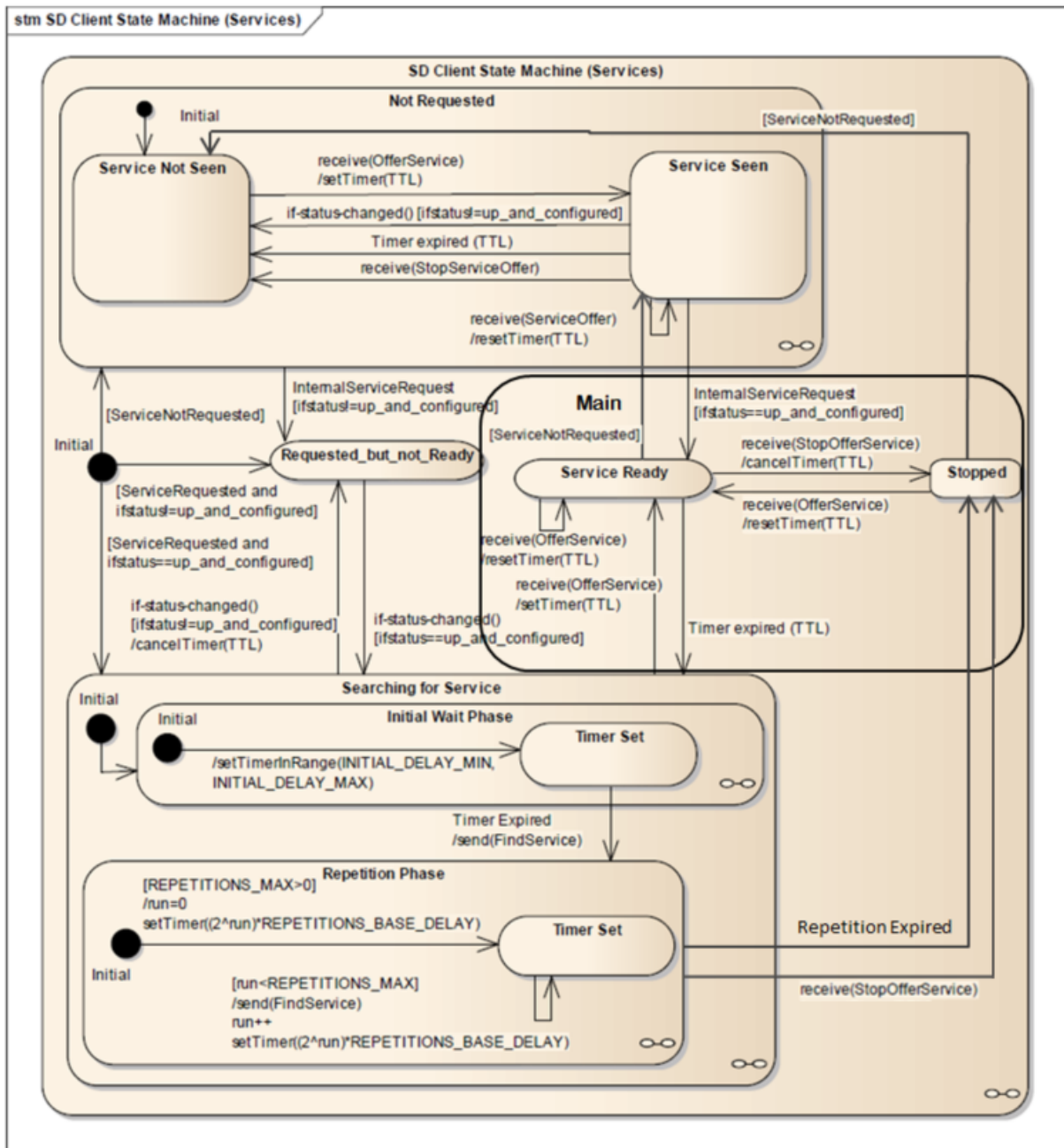
Figure 4.17: SOME/IP Service State Machine Client
