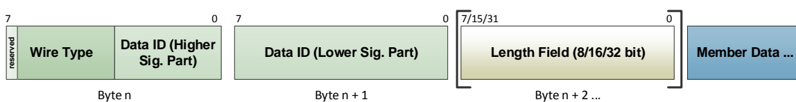
Figure 7.6: SOME/IP Struct Tag Layout
